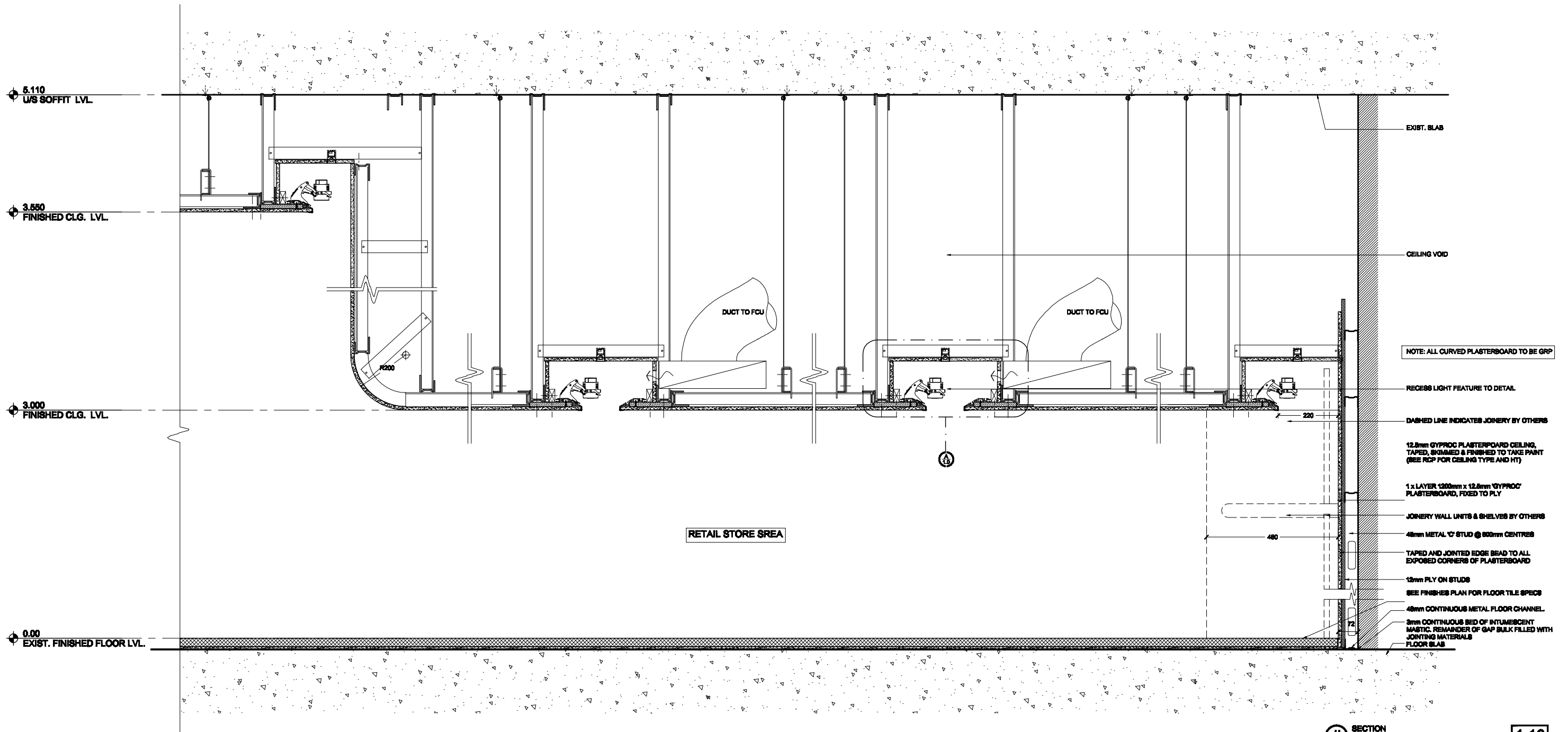
# SECTION TYPICAL CURVED CEILING PROFILE 1:10
